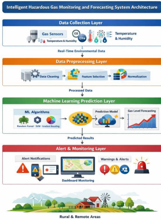
Fig 5.1: Structure of the Proposed System
