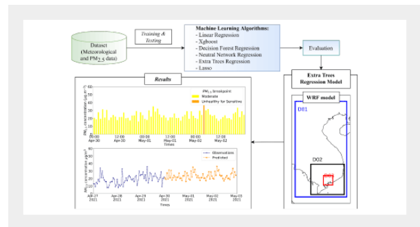
Fig 6.4: Model Training
