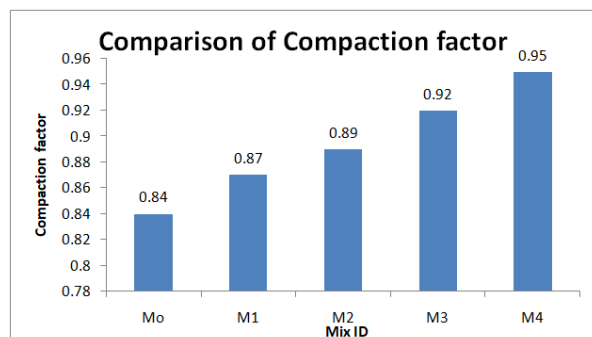
Graph 2: Comparison of compaction factor
