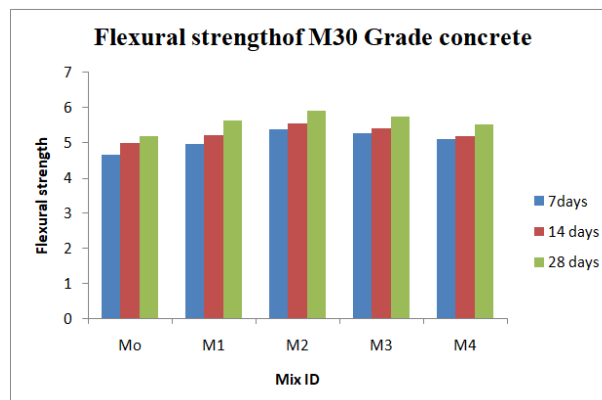
Graph 5: Comparison of Flexural strength
