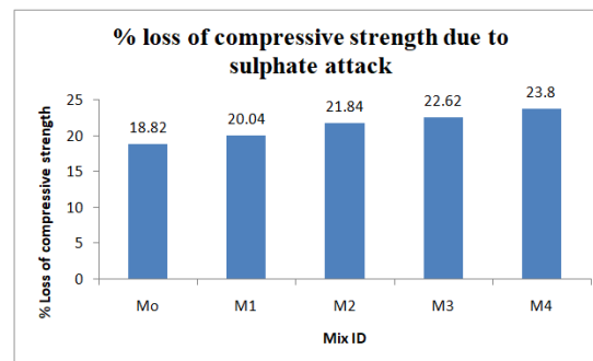
Graph 10: Comparison of percentage loss of strength
