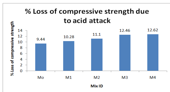
Graph 7: Comparison of percentage loss of strength
