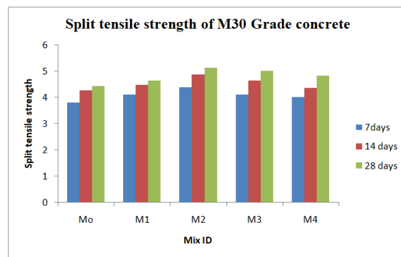
Graph 4: Comparison of Tensile strength
