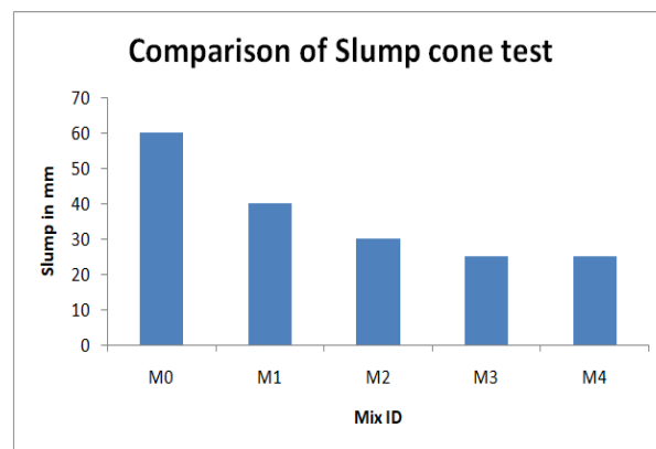
Graph 1: Comparison of slump cone test
