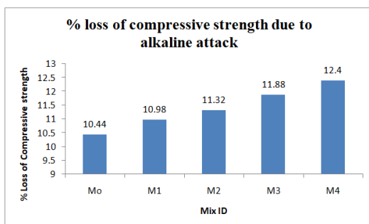
Graph 9: Comparison of percentage loss of strength
