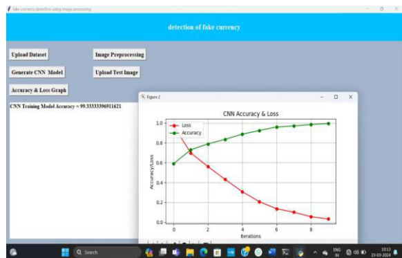
Accuracy and loss Graph' to represent the CNN accuracy and loss graph
