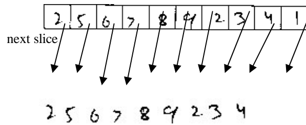
Fig 2.2 Handwritten matching
