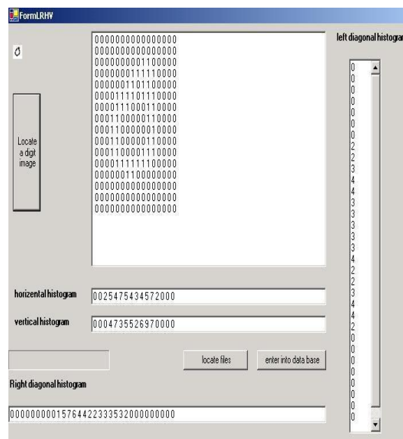
Fig. 2.3 AI Engine Interface
