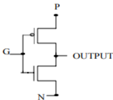
Figure 1.1 Basic GDI cell
