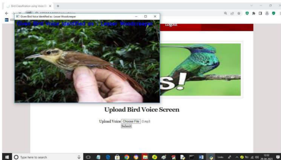
Fig 4. Voice identified
