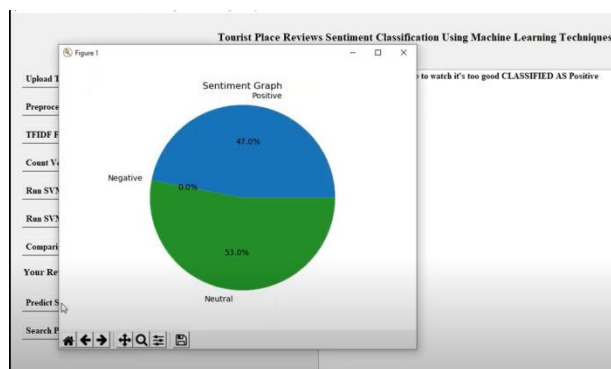
Fig.5. Output results.
