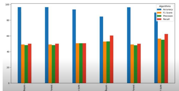
Fig.4. Output graphs.
