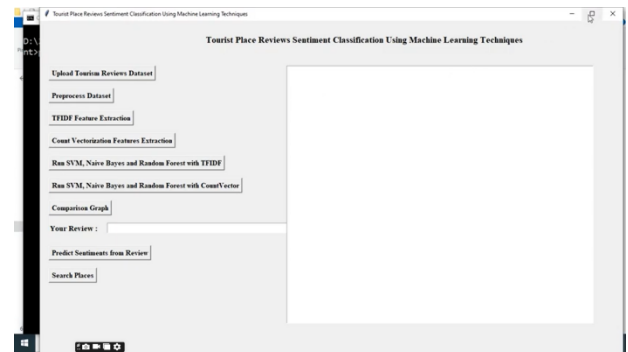
Fig.1. Home page.
