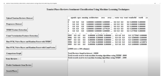
Fig.3. Prediction page.
