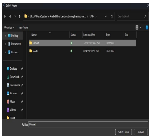
Fig.2. Loading Dataset.
