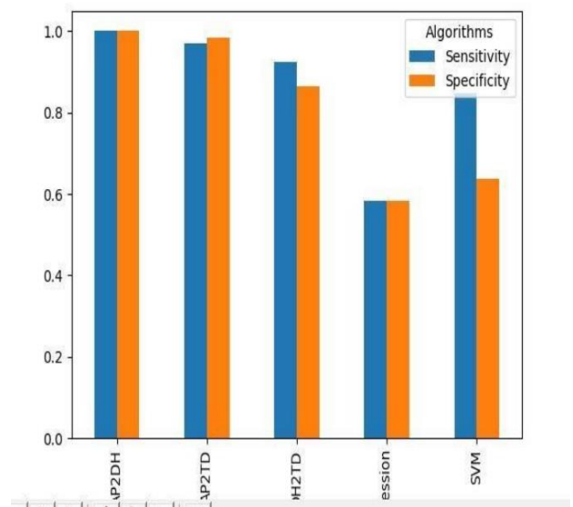
Fig.8. Output Graphs.
