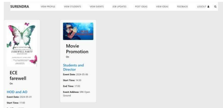
Figure8: View Events
