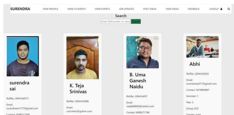
Figure7: View Students
