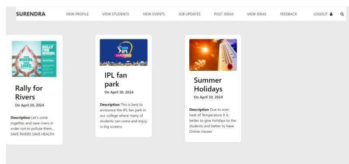
Figure11: View Ideas
