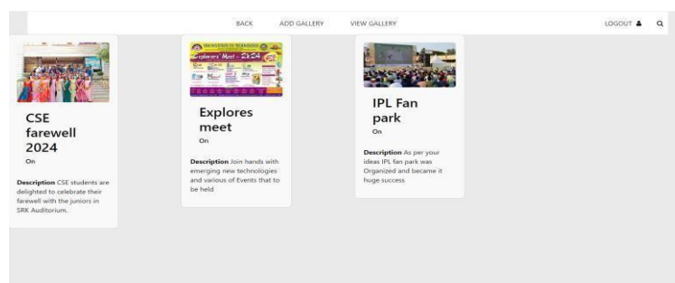
Figure20: View Gallery
