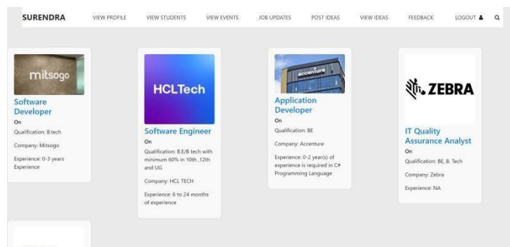
Figure9: Job Updates
