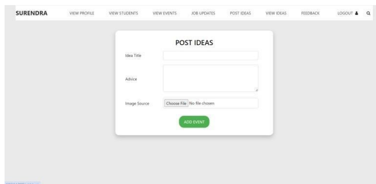
Figure10: Post Ideas
