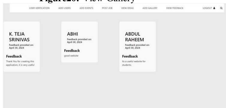
Figure21: View Feedback
