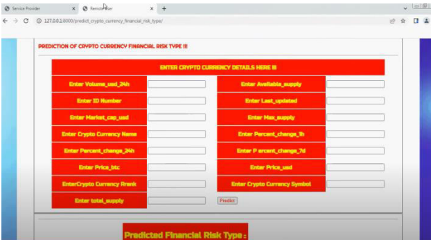
Fig.5. prediction values.
