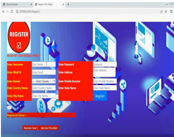
Fig.2. user login
