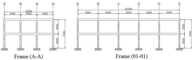
Figure 2: Frame (A-A) and (01-01) of two-story regular RC building (all dimension are in mm)
