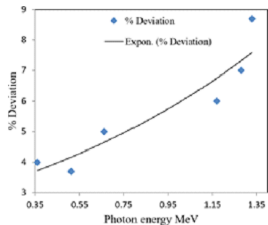
Fig.3: Plots of photon energy versus % deviation of theoretical and experimental values of mass attenuation coefficient of spinel ferrite composite \text{Ni}_{0.5}\text{Mn}_{1.5}\text{Cd}_{0.2}\text{Fe}_2\text{O}_4
